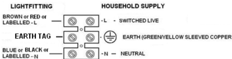
Wiring Details
